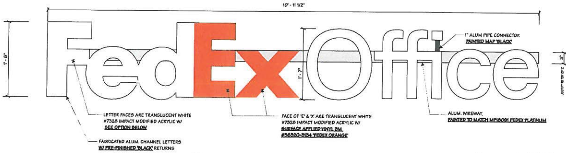
FRONT ELEVATION 1/2" = 1'-0"
